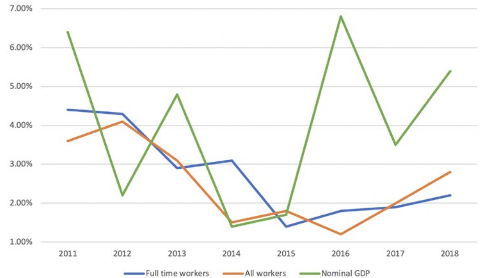
Figure 3: Annual growth in average weekly earnings 26 and nominal GDP 27 , 2011-2018
